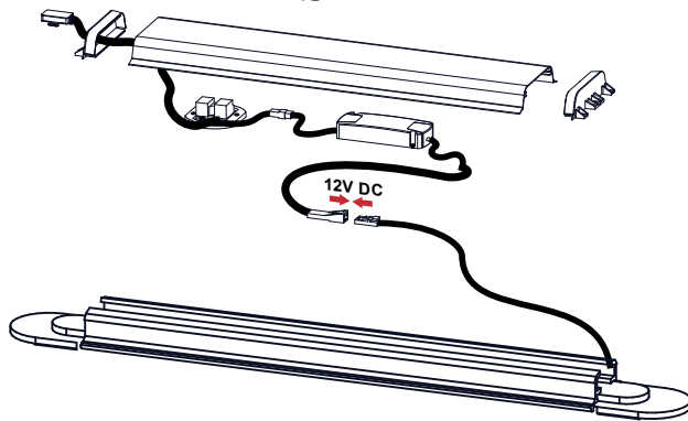
LED SADA TETA LED SET TETA
