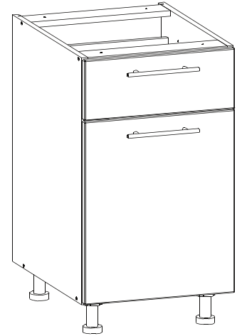
T18 500x520x820
