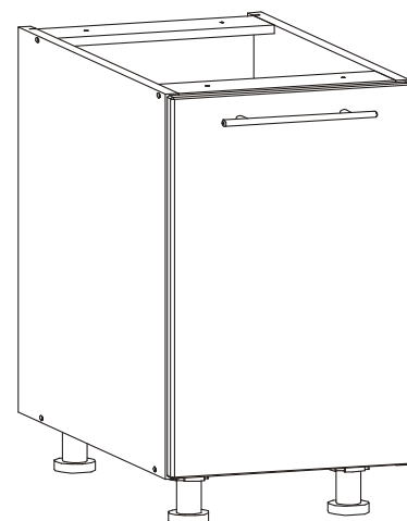
T19 600x520x820
